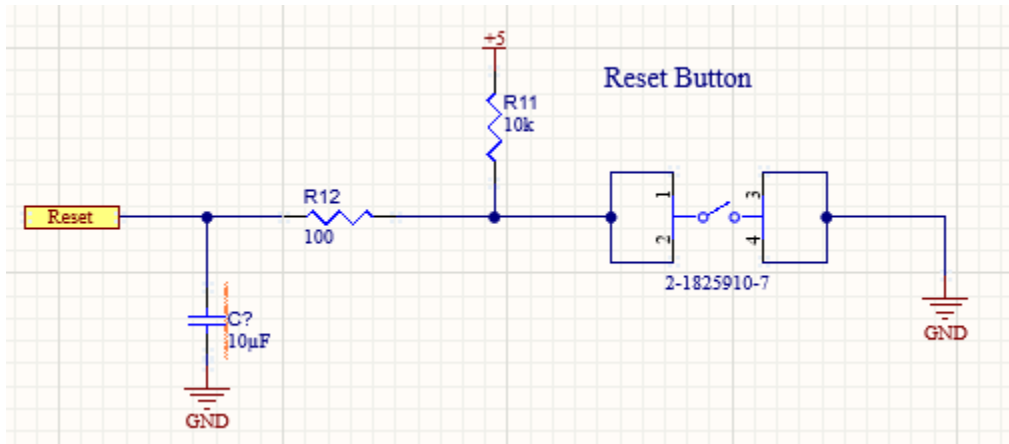
Figure 38. Reset Button Schematic
