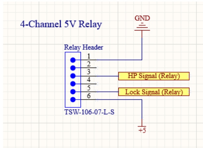
Figure 30. 4-channel 5V Relay Schematic
