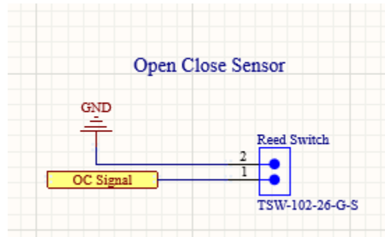
Figure 32. Open Sensor Schematic
