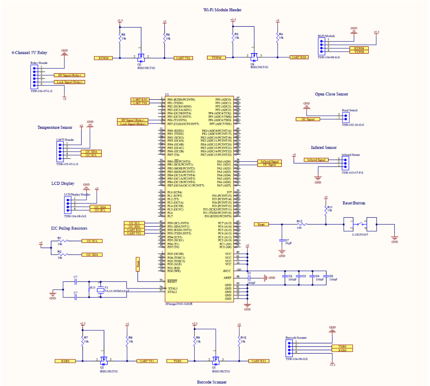
Figure 39. Overall PCB Design Schematic
