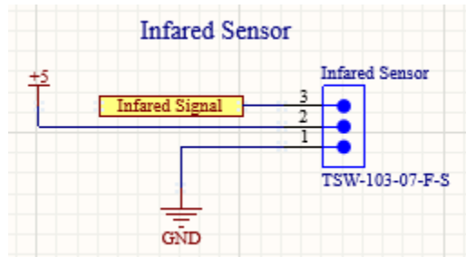
Figure 36. Infrared Sensor Schematic
