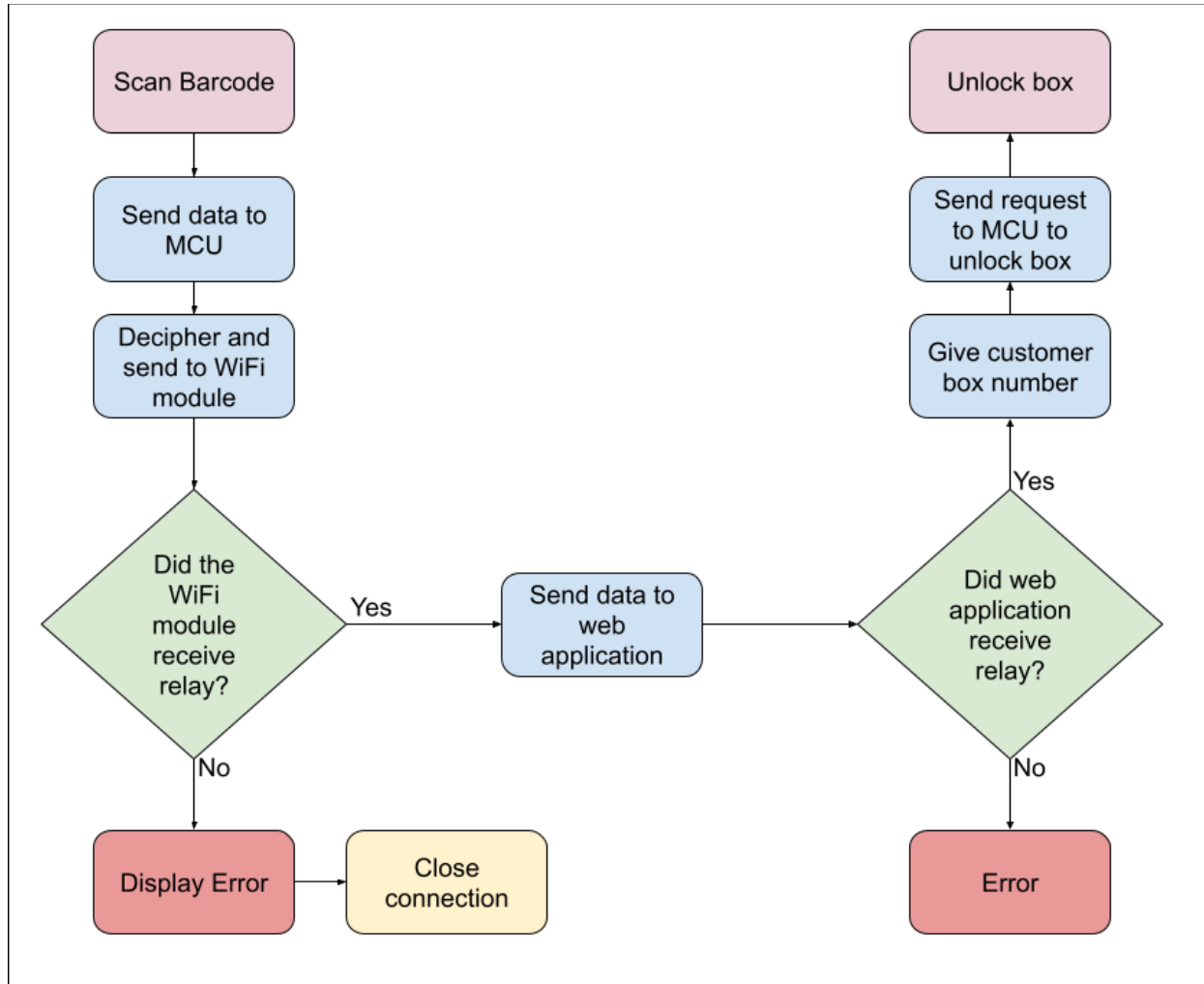
Figure 40: Barcode Scanner Flowchart
