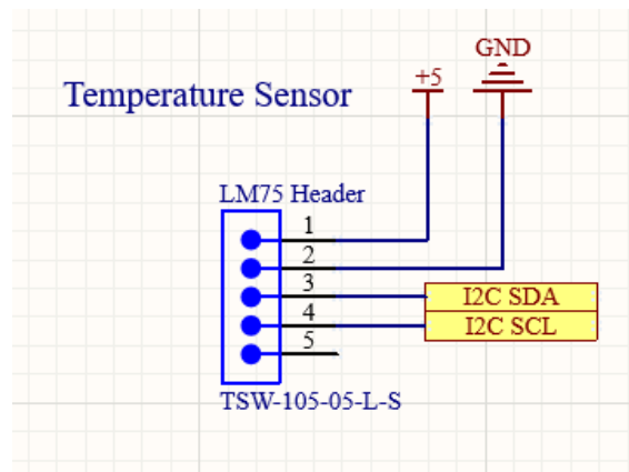
Figure 33. Temperature Sensor Schematic
