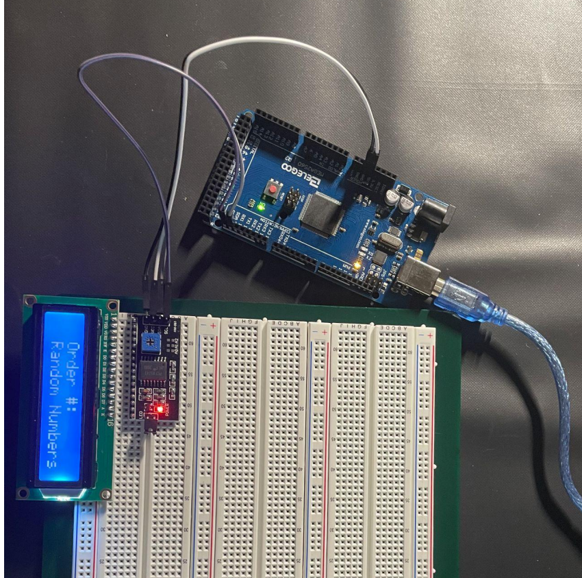
Figure 52. LCD Display Wiring and Testing
