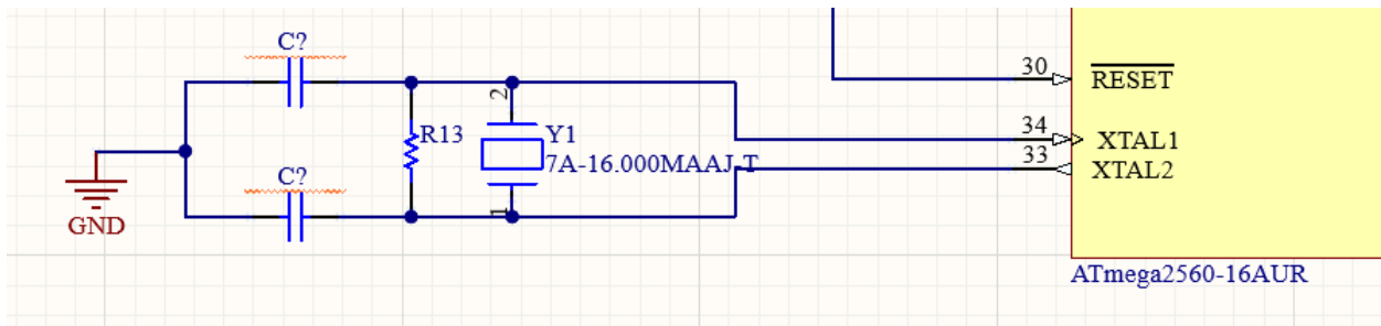
Figure 37. External Clock Configuration Schematic
