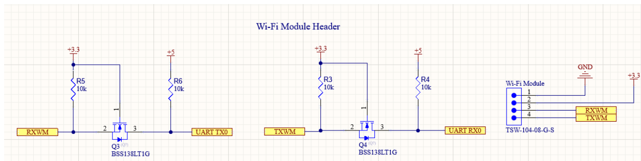
Figure 31. ESP32 Schematic
