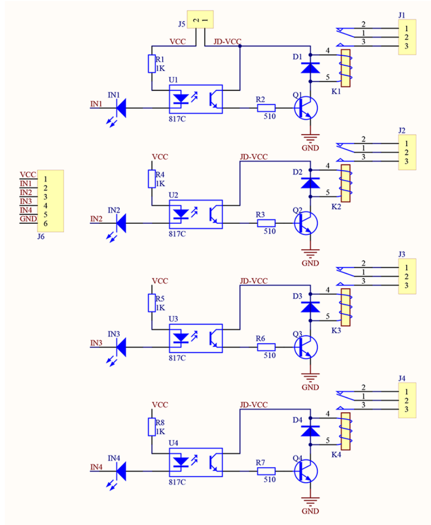
Figure 27: Relay Circuit Diagram
