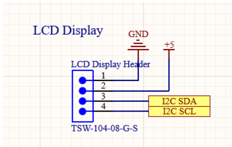
Figure 35. LCD Display Schematic
