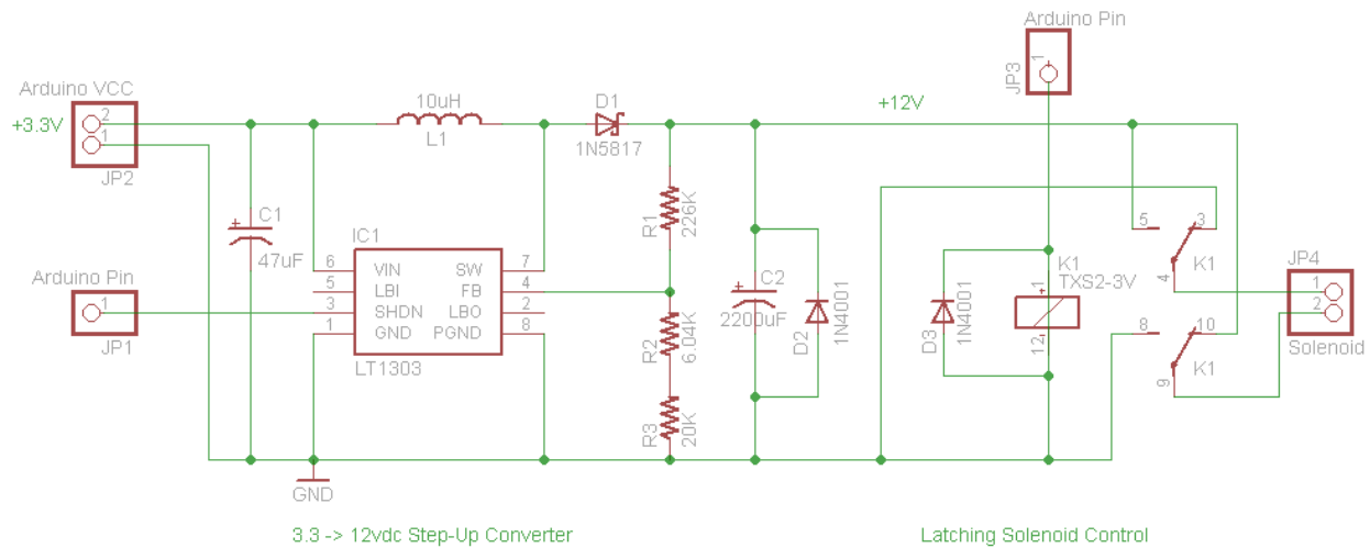
Figure 22. Solenoid Lock Internal Schematics
