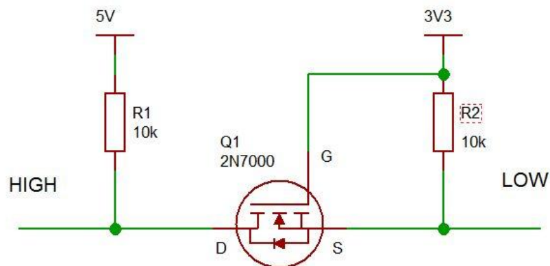
Figure 28. MOSFET Logic Level Conversion Circuit
