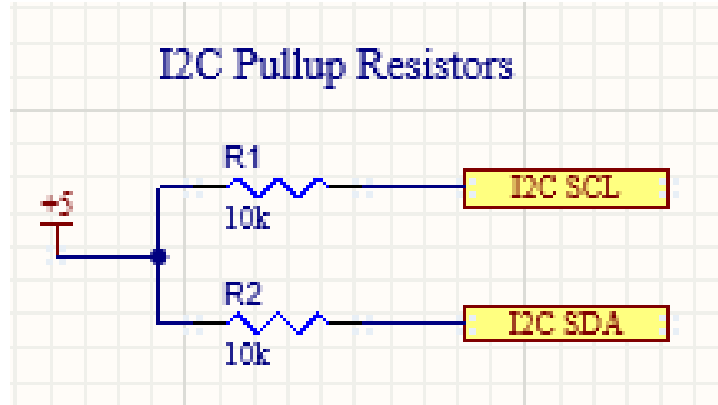
Figure 34. Pull-Up Resistors
