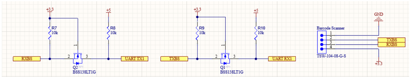
Figure 29. Barcode Scanner Schematic
